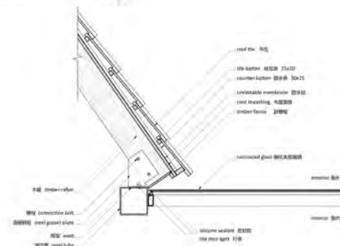
LVL ROOF
