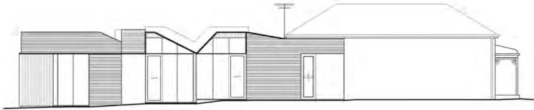
02 NORTH ELEVATION SCALE 1/8"
