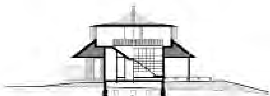
SECTION A
